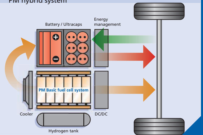
PM hybrid system
